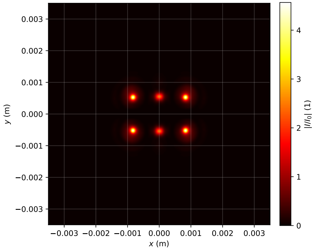
Intensity profile I(x, y, z = 0.637)/I_0 , P_{in}=9.0P_{cr} , artificial time
